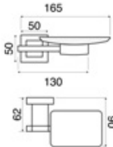
Sabunluk Soap Holder Siyah / Black PLB1084
