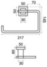
Yuvarlak Havluluk Towel Ring PL1003
