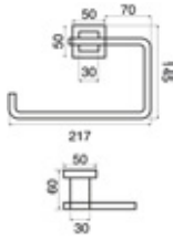
Yuvarlak Havluluk Towel Ring Mat Bronz / Mat Bronze PLM1053
