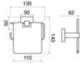
Kağıtlık Paper Holder Mat Bronz / Mat Bronze PLM1050
