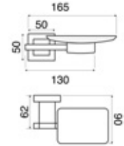
Sabunluk Soap Holder Mat Bronz / Mat Bronze PLM1054
