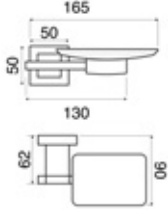
Sabunluk Soap Holder PL1004
